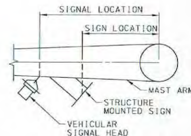
ANGLED SIGNS AND SIGNAL MEASUREMENT DETAIL
